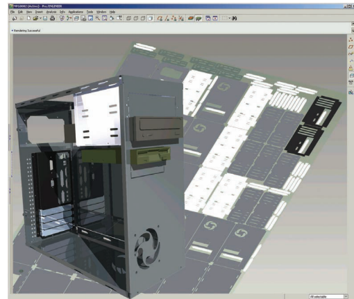
AutoNesting in Pro/ENGINEER NC Sheetmetal Option helps you maximize your use of the sheet area.
